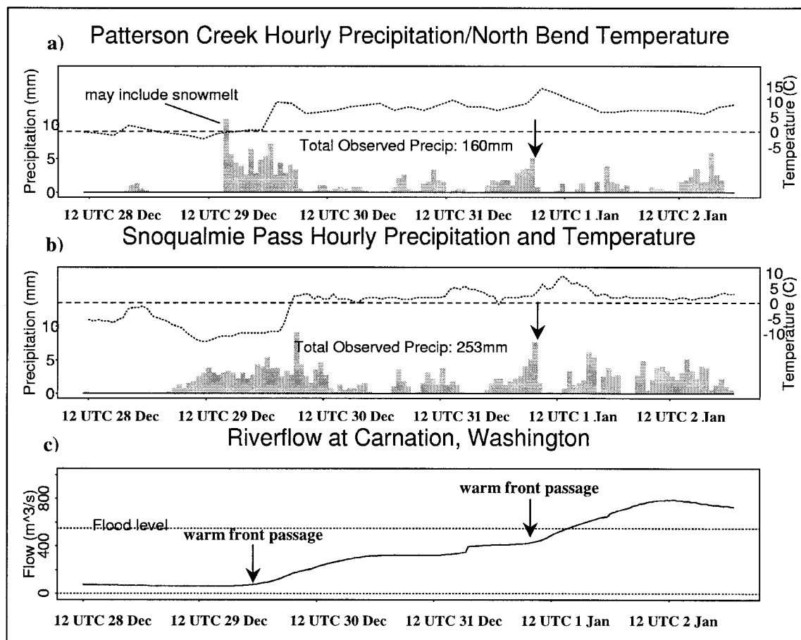
FIG. 6. Observed hourly precipitation at (a) Patterson Creek and (b) Snoqualmie Pass, temperatures (dotted) from (a) North Bend and (b) Snoqualmie Pass, and (c) observed river flow on the Snoqualmie River at Carnation.
